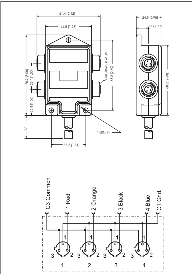
Dimensional data
