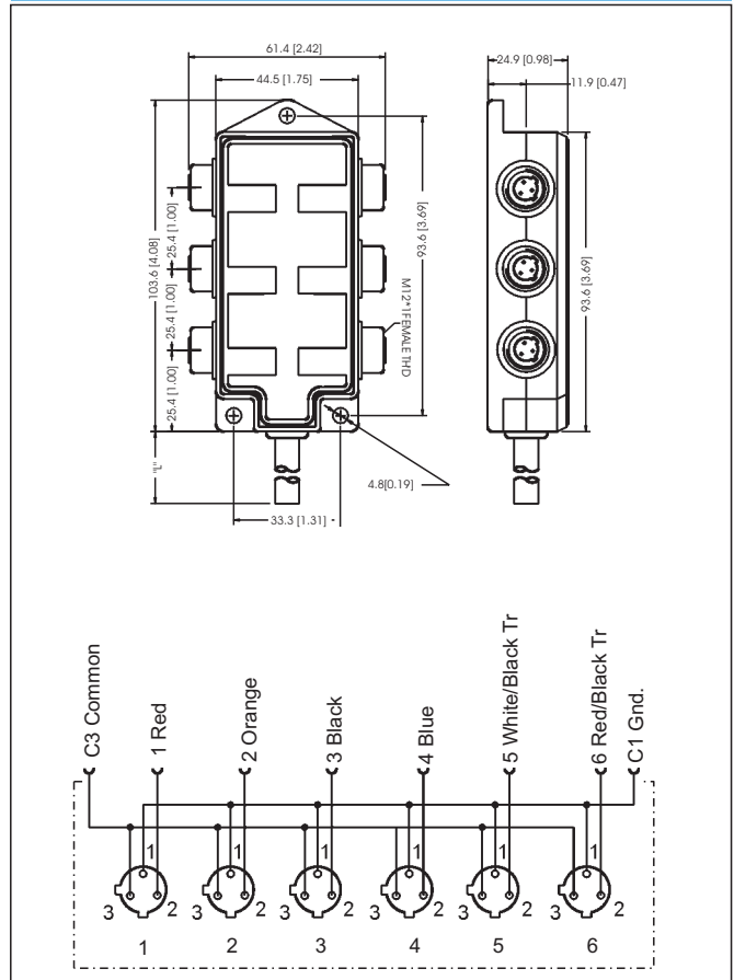
Dimensional data
